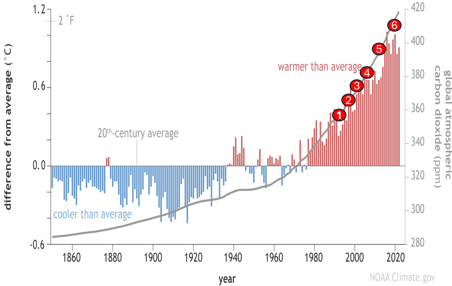
Yearly global surface temperature and atmospheric carbon dioxide (1850-2022)
